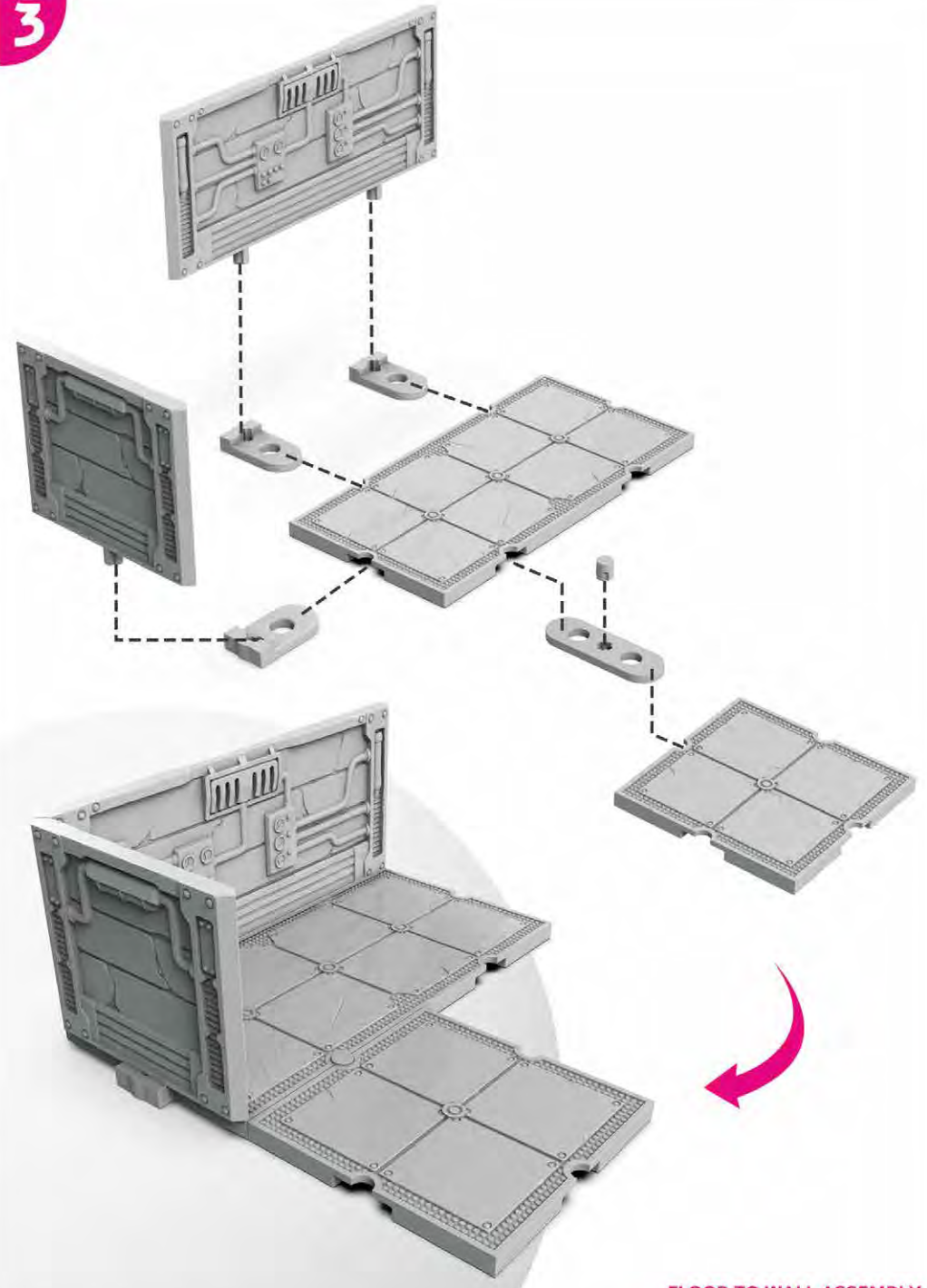
FLOOR TO WALL ASSEMBLY
